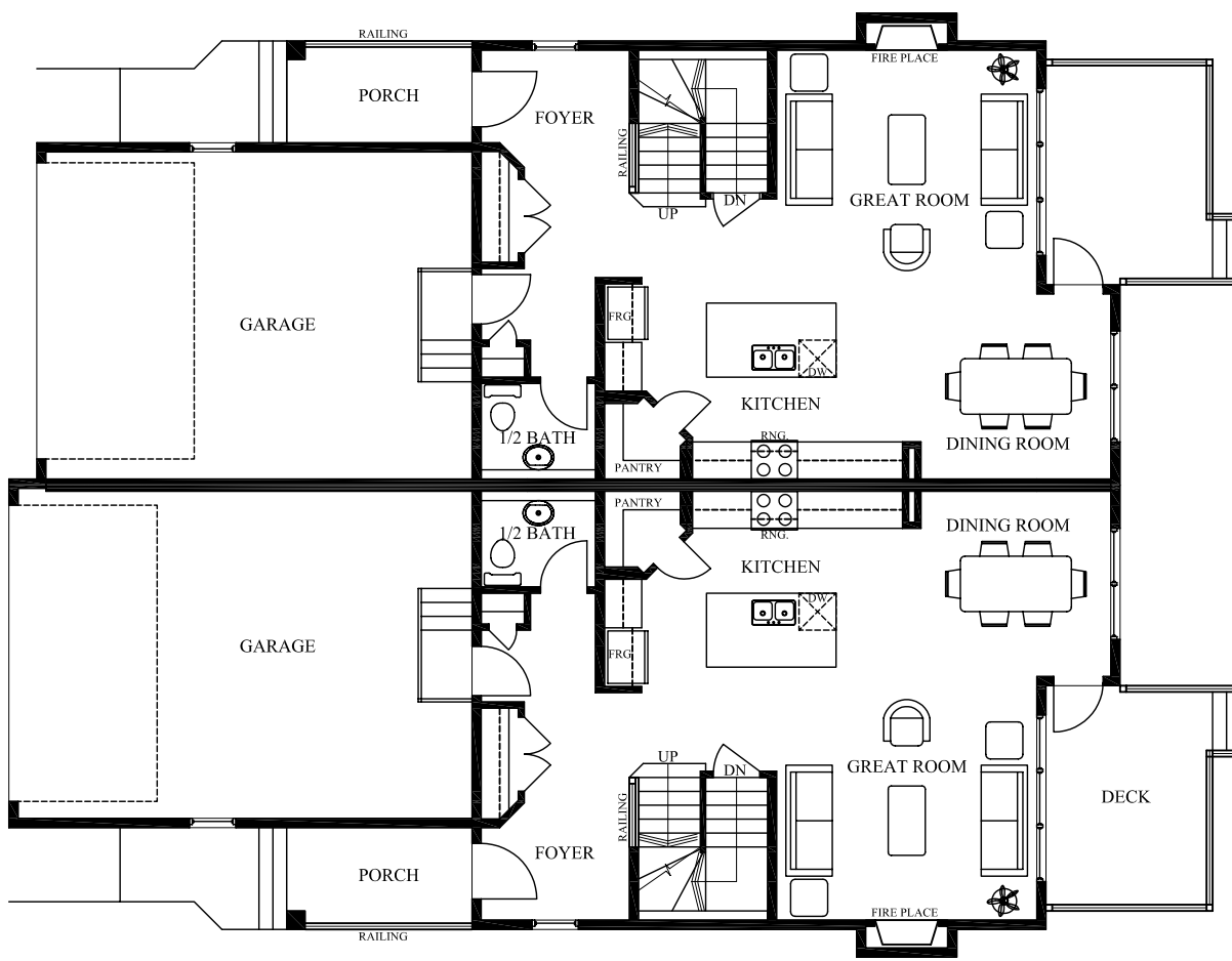
MAIN FLOOR PLAN 787 Sq.ft.
