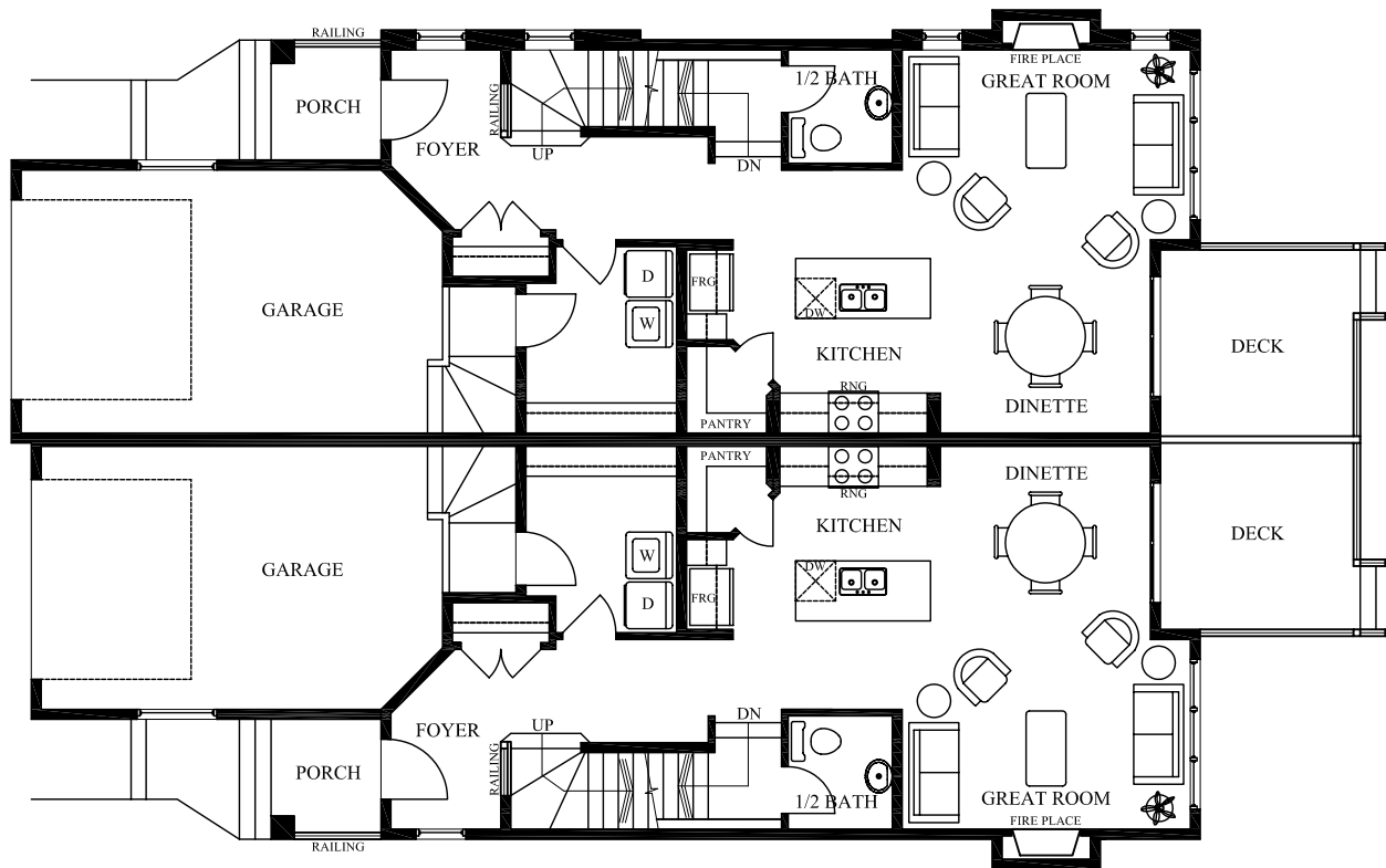
MAIN FLOOR PLAN 741 Sq.ft.
