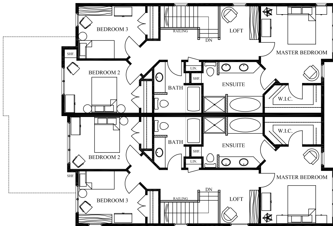
SECOND FLOOR PLAN UNIT 5803: 891 Sq.ft. UNIT 5805: 880 Sq.ft.
